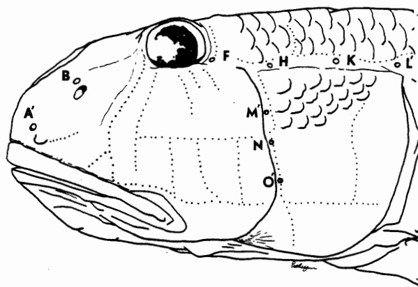
Fig. 3. Cephalic sensory papillae and lateralis canal pores of Gobionellus oceanicus , NLU 3201, 127.5 mm SL. Pore labels as in Fig. 2. Pores C and D not shown.
