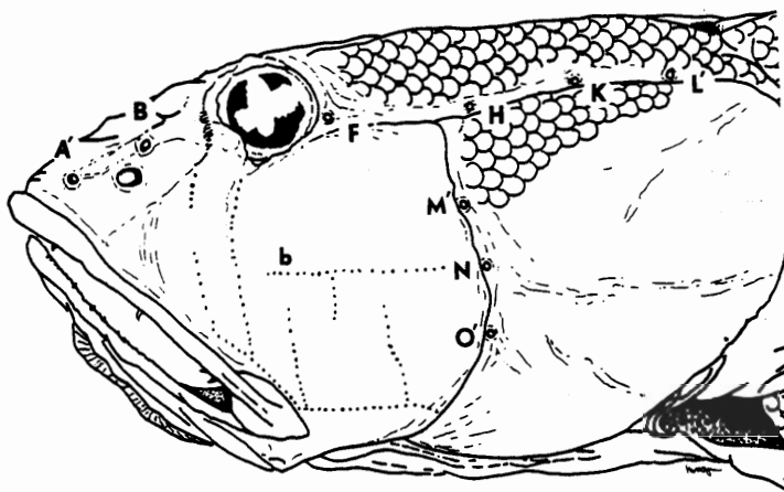
Fig. 2. Cephalic sensory papillae of the cheek region and lateralis canal pores on the holotype of Paroxyrichthys typus , 85.5 mm SL. Pore terminology as in Akihito et al. (1984). Pores C and D not shown. "b" indicates longitudinal papillae row b (Miller and Wongrat, 1979).
